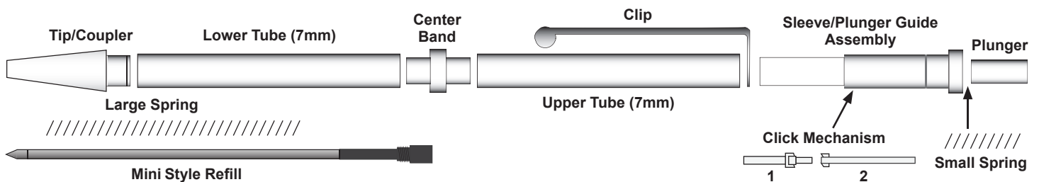
Diagram A - Pen Parts and Assembly
