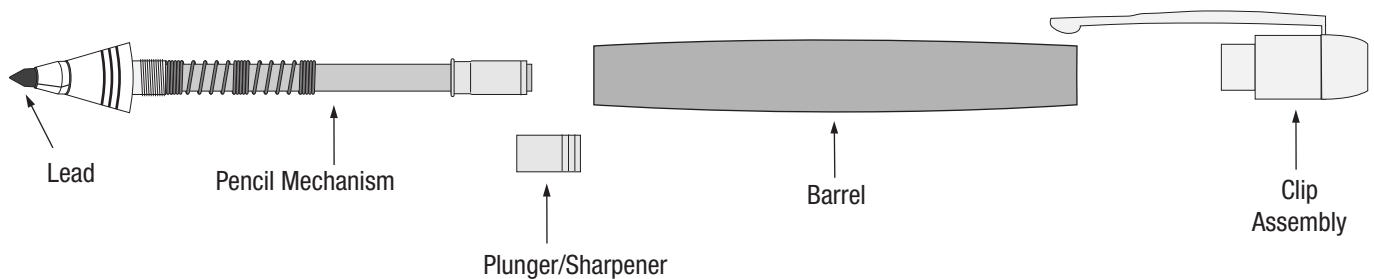
DIAGRAM C • Assembly
