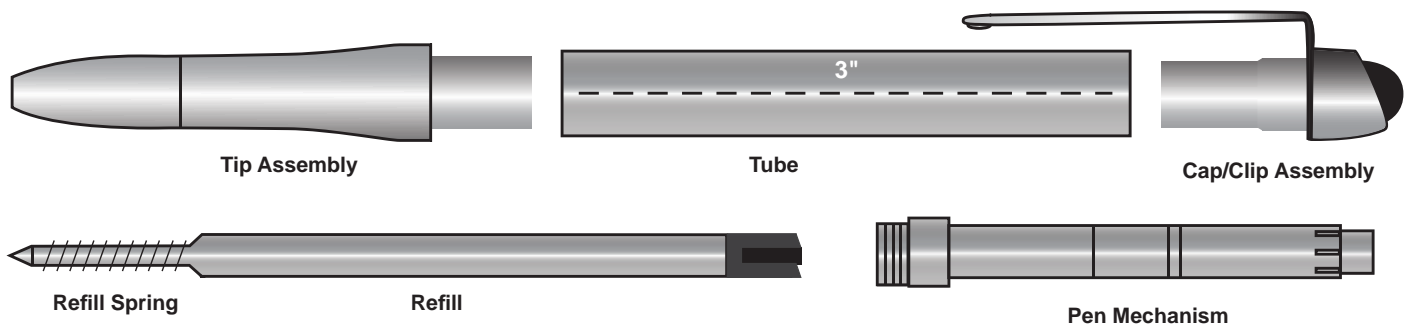
Diagram A - Parts and Assembly
