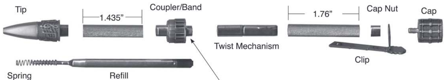
DIAGRAM A / PARTS LAYOUT
