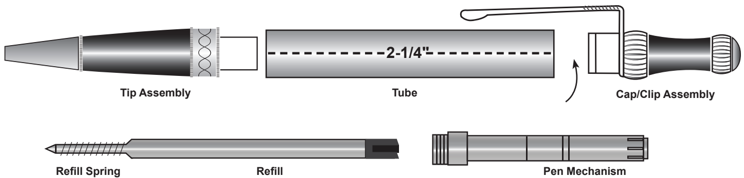
Diagram A - Parts and Assembly
