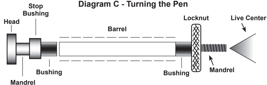
Diagram C - Turning the Pen
