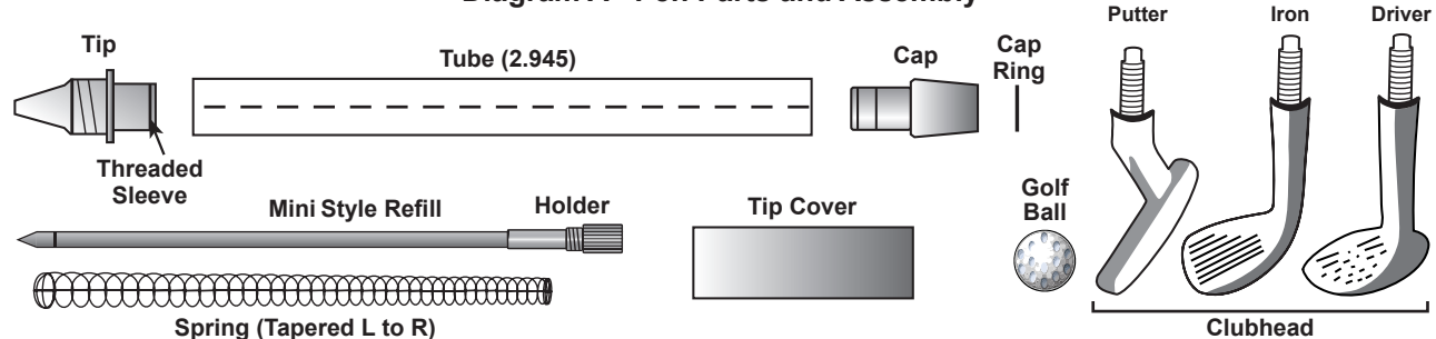
Diagram A - Pen Parts and Assembly
